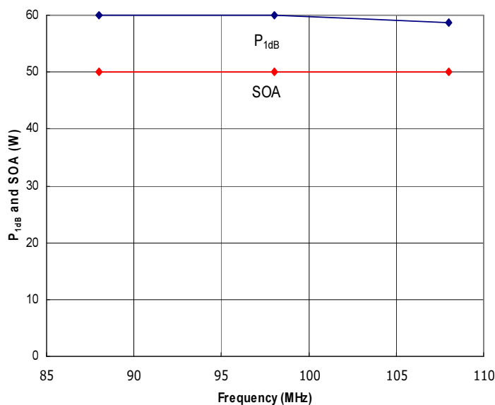
Figure 4: RFP88-108-50 Typical P 1dB and Safe Operating Area (SOA).
