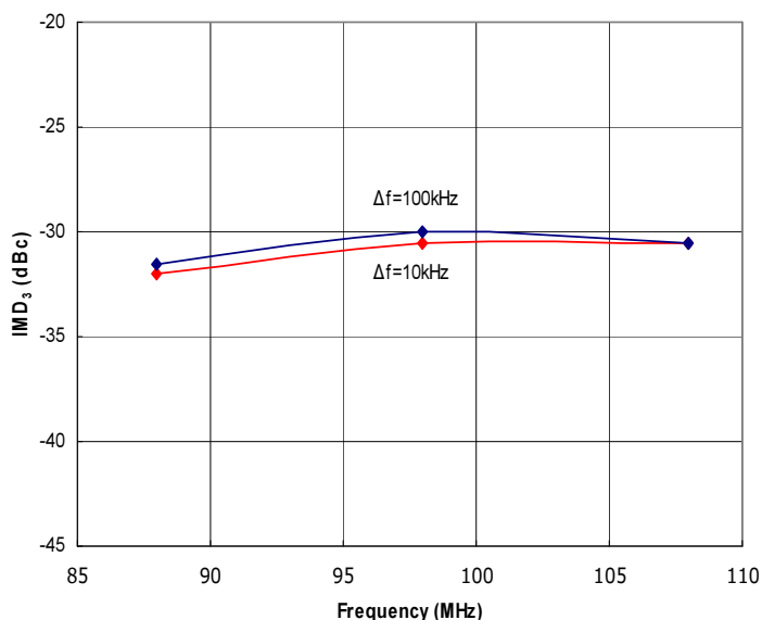
Figure 2: RFP88-108-50 Typical IMD 3 , Δf=10kHz and 100kHz, @ P out = 50W PEP. Data is provided for reference only; this is not intended to be a linear amplifier. For improved linearity, see our RFP88-108-25 Class A amplifier.
